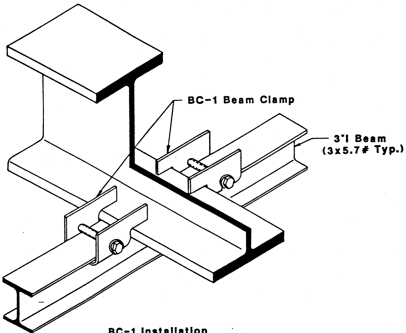
BC-1 Installation
