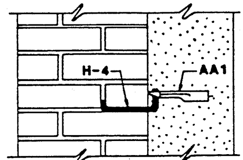
Solid Sidewall
