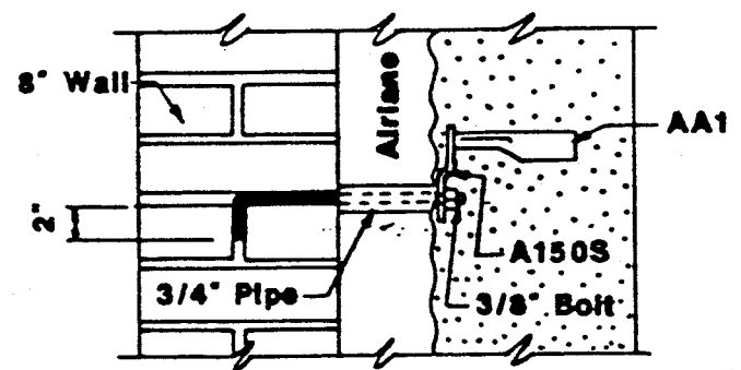
Air Cooled Sidewall
