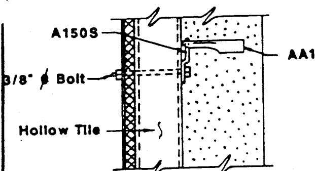
Steel Cased Sidewall
