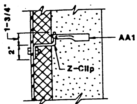
Steel Cased Sidewall
